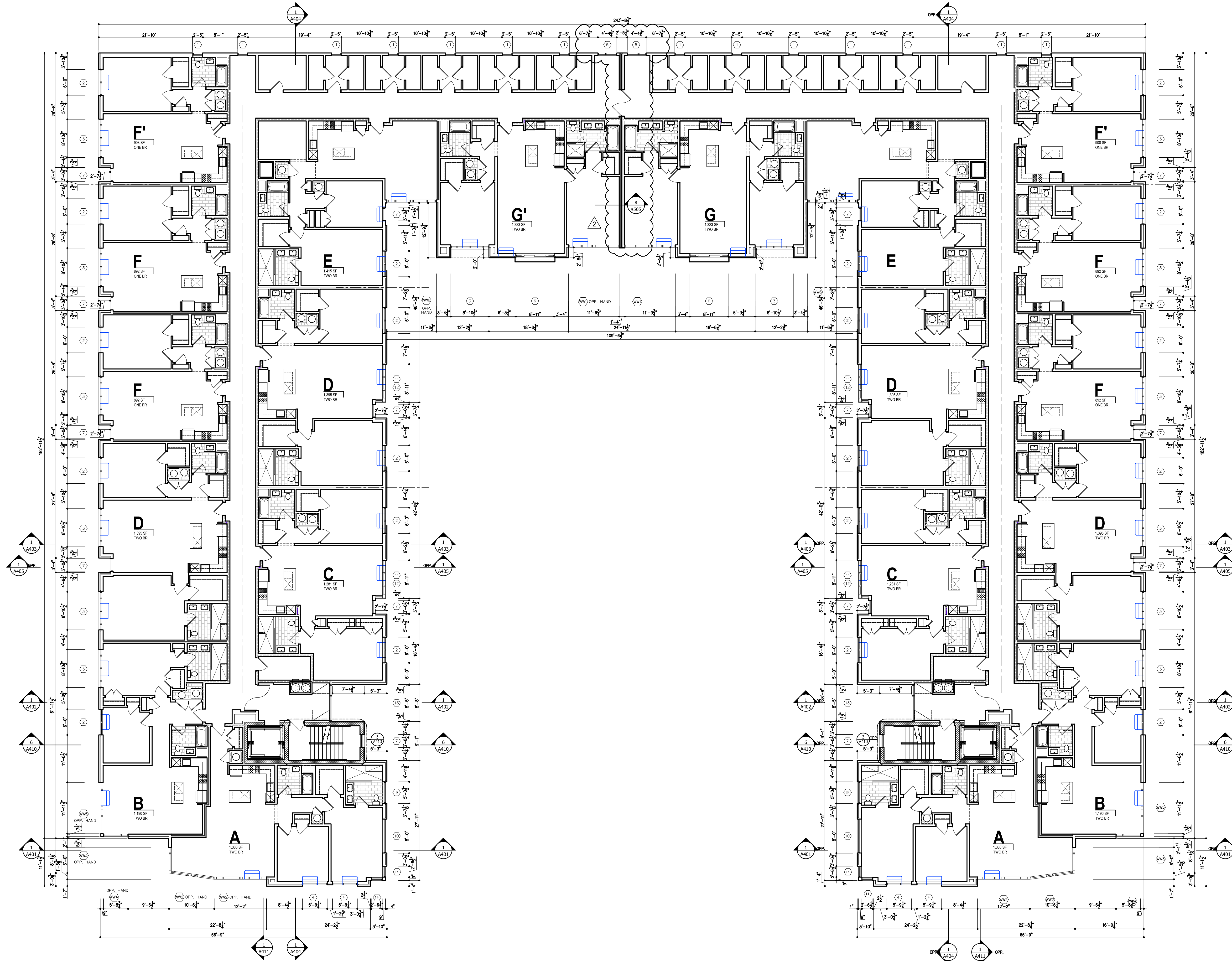
1 Residential Floor Plan R2 A103 3/32" = 1'-0"
