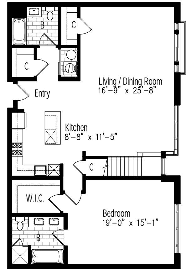
Lower Floor
