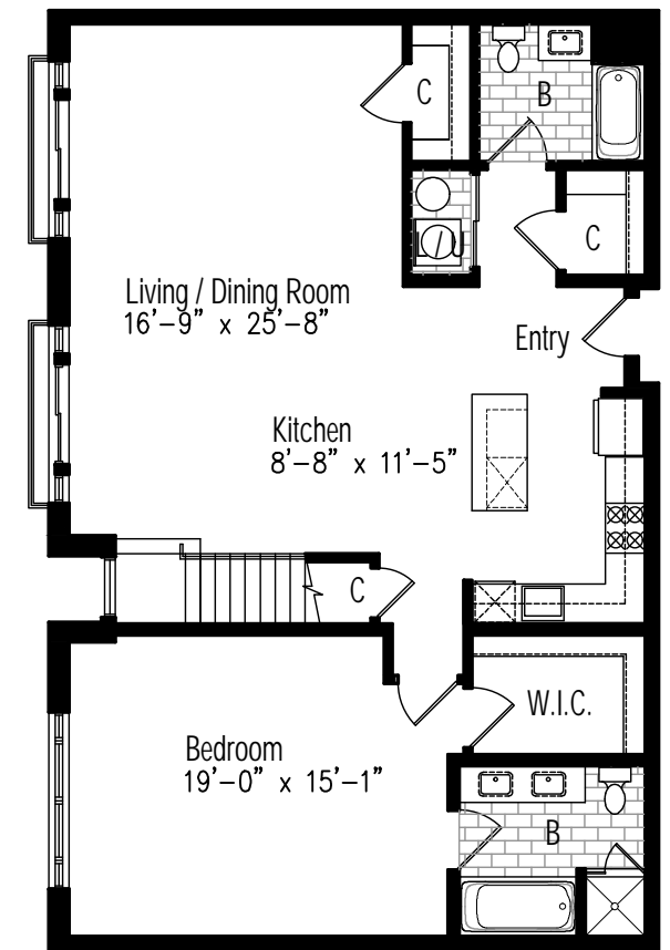
Lower Floor
