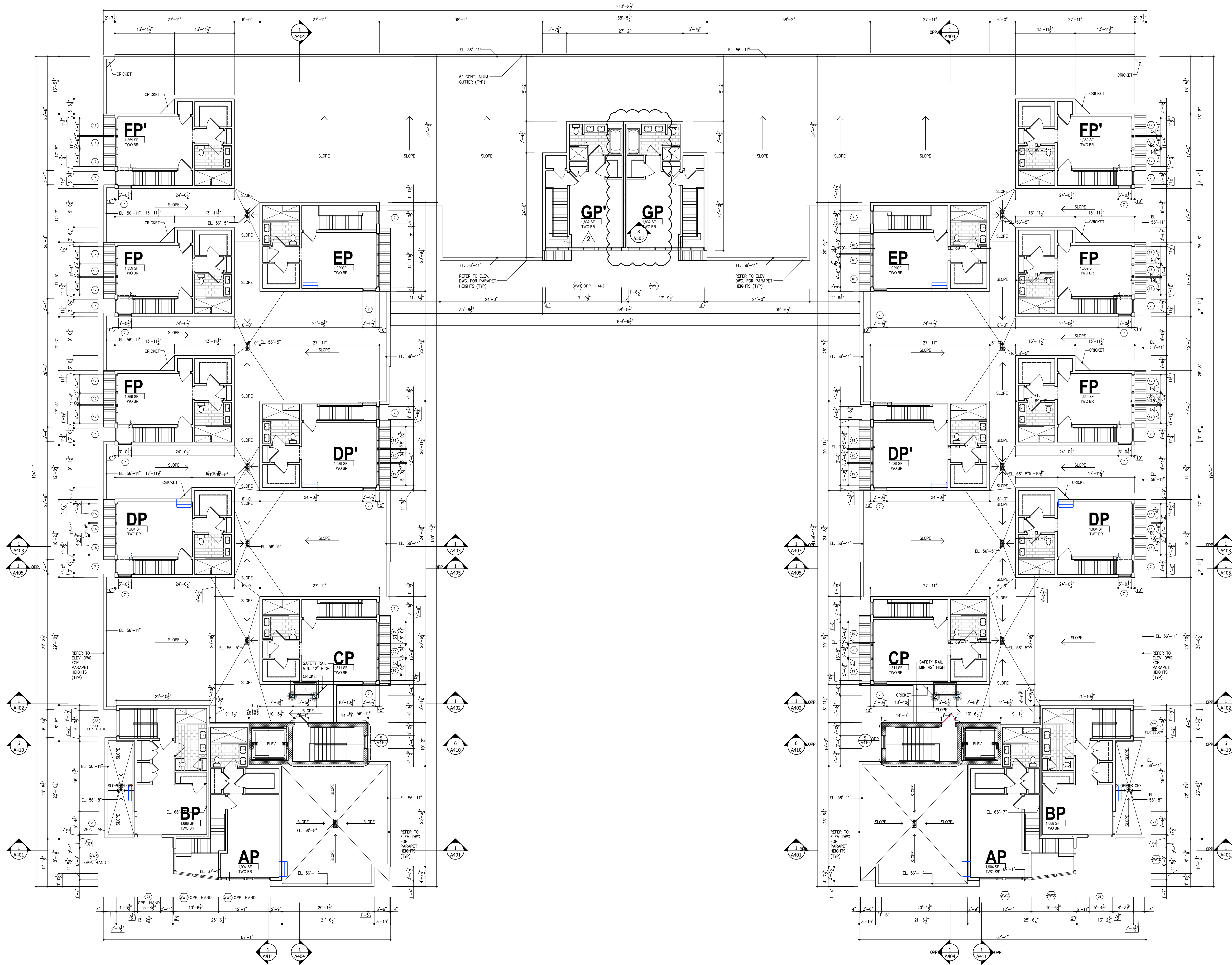
1 Residential Floor Penthouse 3/32" = 1'-0"
