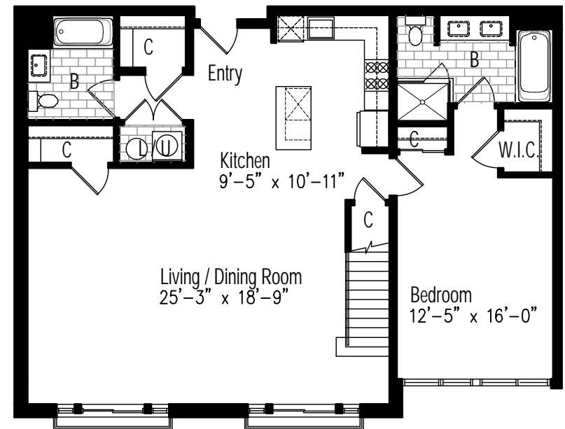
Lower Floor
